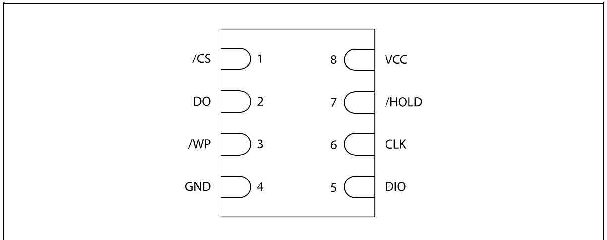
Figure 1b. W25X16 Pad Assignments, 8-pad WSON (Package Code ZP)
